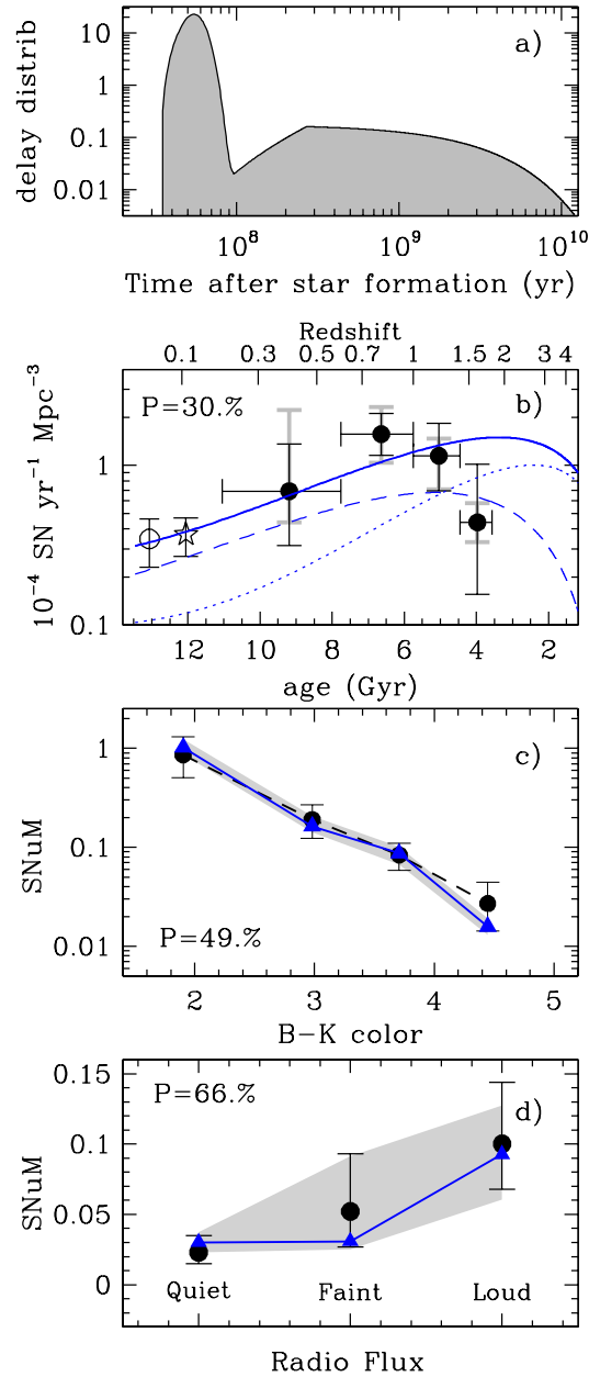
FIGURE 1. The SN rates for a DTD constituted by equal contributions (50%) of an exponentially declining function with e-folding time of 3 Gyr and a gaussian centered at 5 \times 10^7 yr and \sigma = 10^7 yr. Panel (a): the DTD itself (number of SNIa per unit time after star formation); Panel (b): the evolution of the rate along the cosmic age. The solid curve is the prediction for the considered DTD. Data are from Mannucci et al. (2005; open circle), Strolger et al. (2004; star), Dahlen (2004; dots, with black error bars for 1\sigma statistical errors, and the gray bars for systematic uncertainties). In panel (b) the dotted and dashed lines show the contributions from the “prompt” and “tardy” components, respectively. P is the statistical probability of agreement estimated from the statistical errors only. Panel (c): the predictions (solid line and triangles) for SNIa rates as a function of the parent galaxy (B–K) colour, expressed in SNe per century per 10^{10} M_{\odot} of stellar mass (SNuM). The dots and the dashed line show the observational data from Mannucci et al. (2005). Panel (d): SNIa rates in early-type galaxies as a function of the radio power of the parent galaxy. The black dots are the observed SN rates in Della Valle et al. (2005) with 1\sigma Poisson error.
